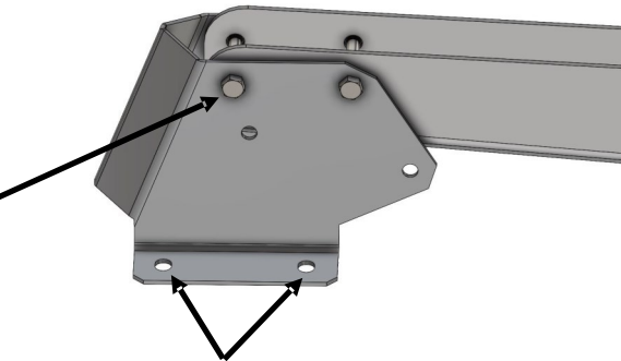
Studs at top of heater to mounting bracket
