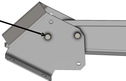
Studs at top of heater to mounting bracket
